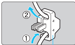
Clamp
